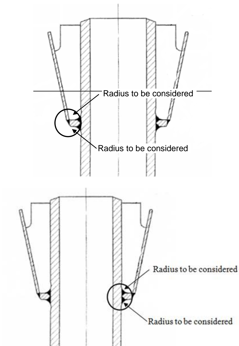
Figure 9 Fillet shoulder radius
