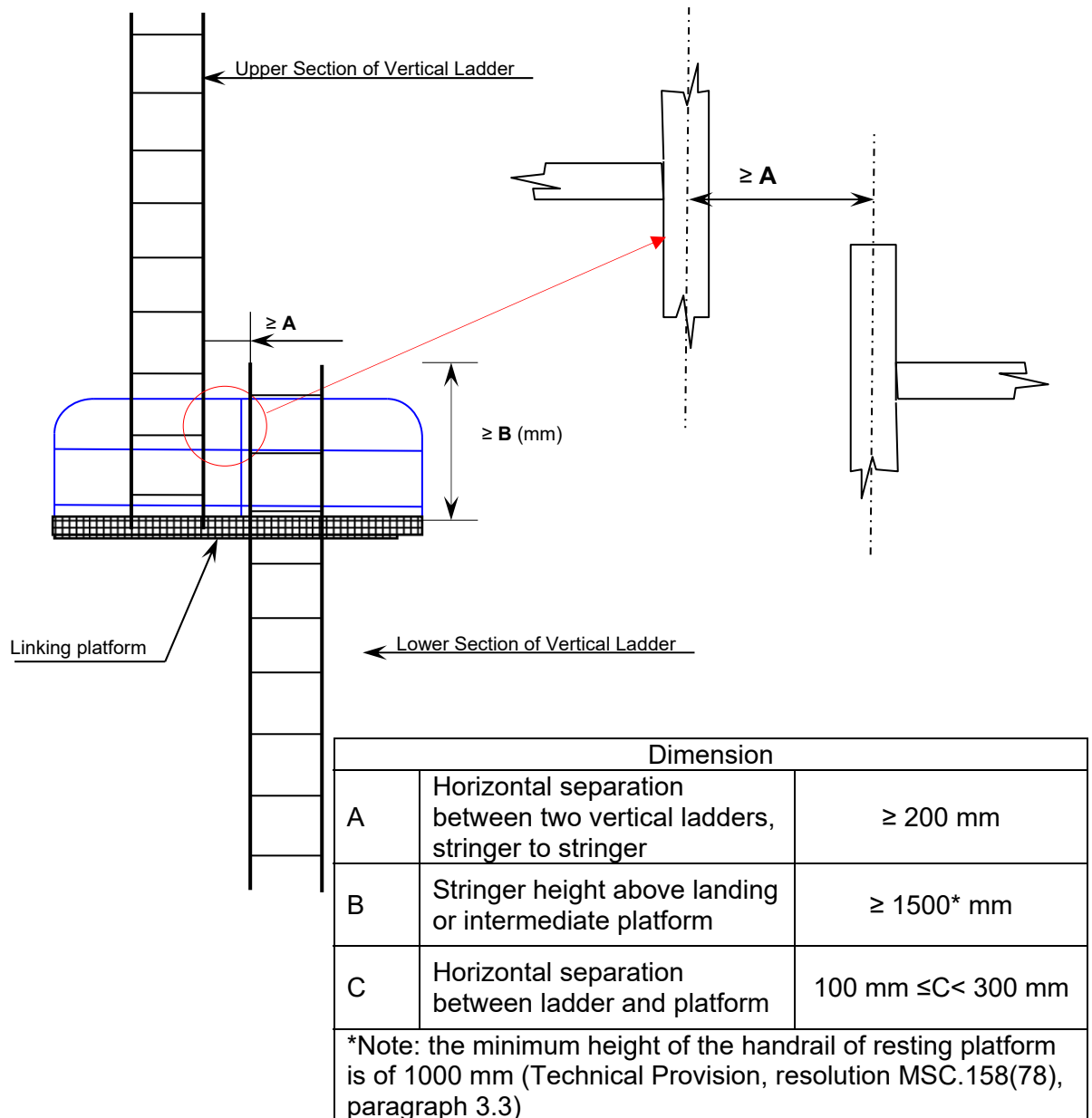
Figure "A" Vertical Ladder – Ladder through the linking platform
