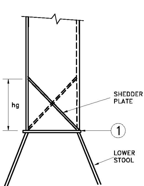
Figure 3a Symmetric shedder plates
