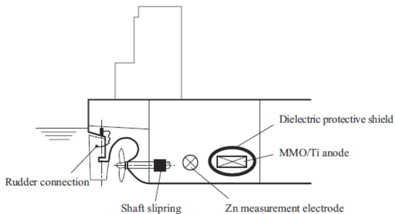
Figure 22.4 Schematic arrangement of an impressed current system (stern area)
