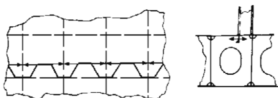
Figure 3.3 Corrugated bulkhead support
