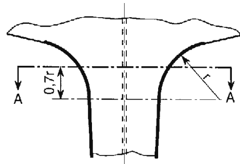
Figure 10.8 Transition between rudder horn and shell
