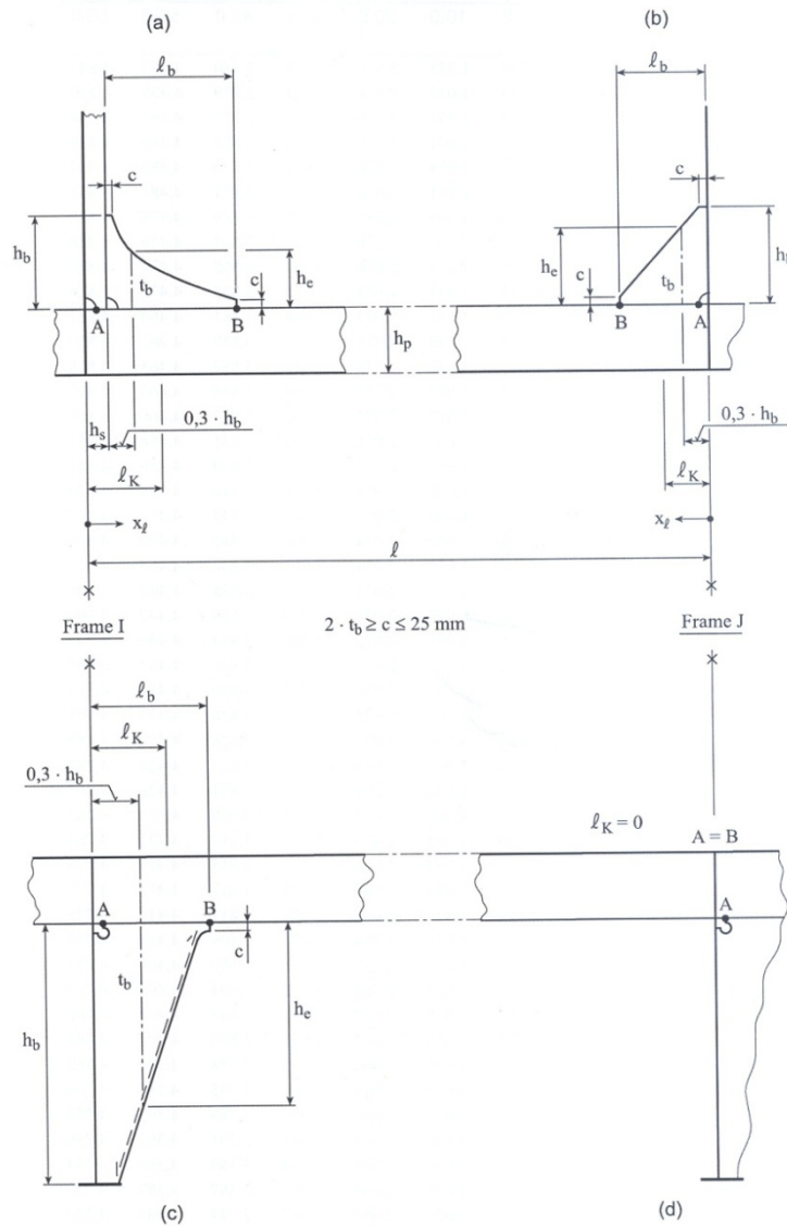
Figure 8.5 End attachment
