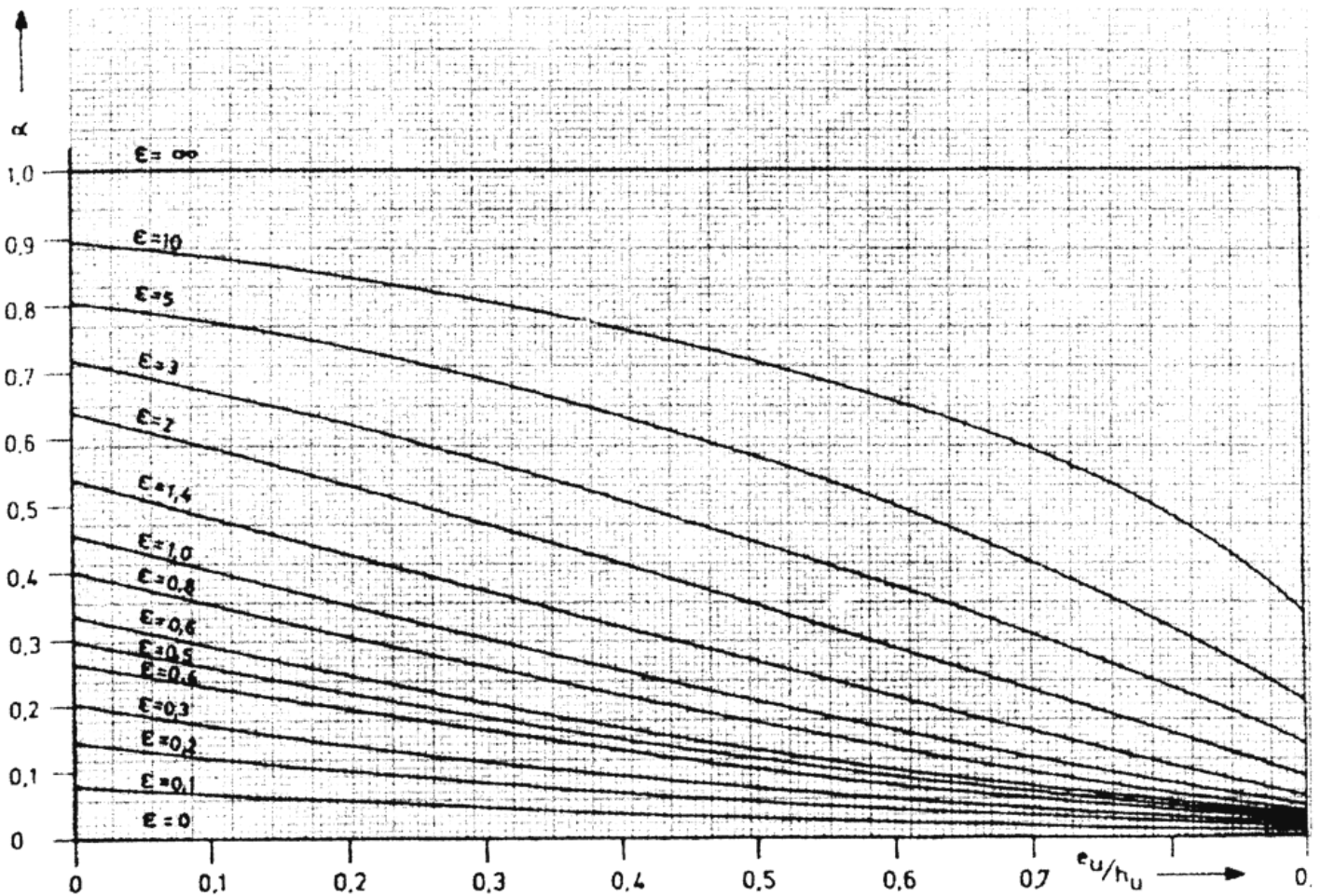
Diagram 8.1 coefficient \alpha
