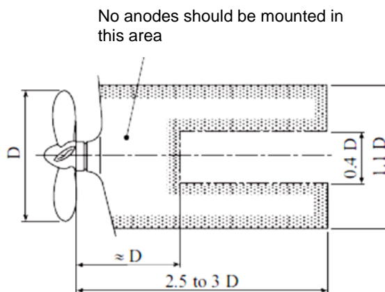
Figure 22.2 Anode-free zones in way of the propeller
