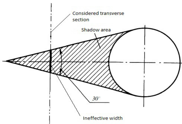
Figure 6.7 Shadow area
