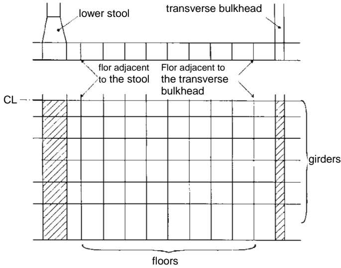
Figure 27.9 Girders and floors in the double bottom
