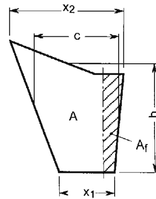
Figure 18.1 Rudder area geometry
