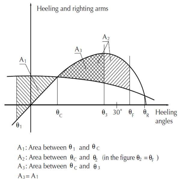
Figure 26.3 Cargo loss
