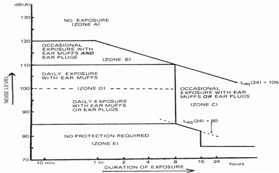
Figure 2.1 Allowable daily and occasional noise exposure limits
