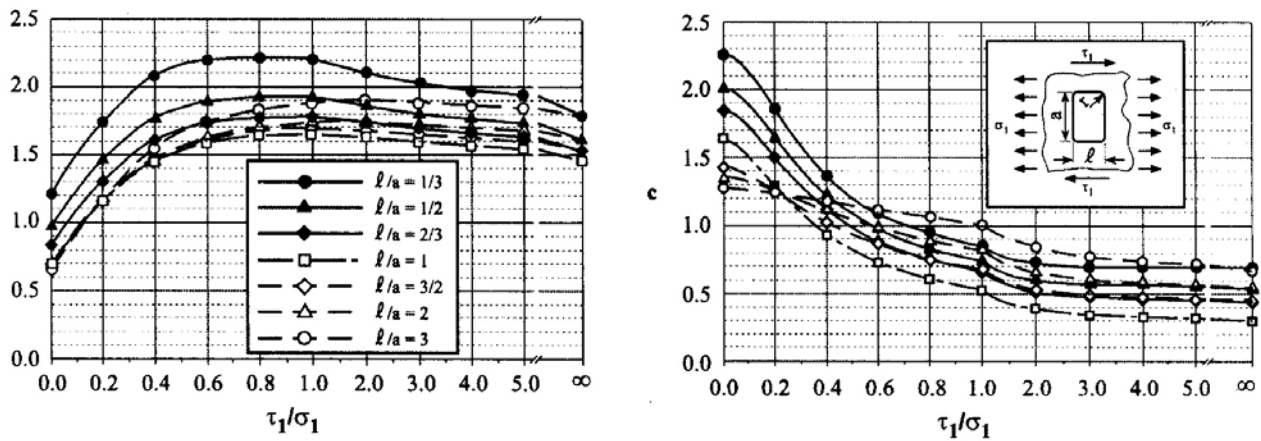
Figure 3.10 Parameters m and c to determine the notch factors of rectangular openings loaded by superimposed longitudinal and shear stresses
