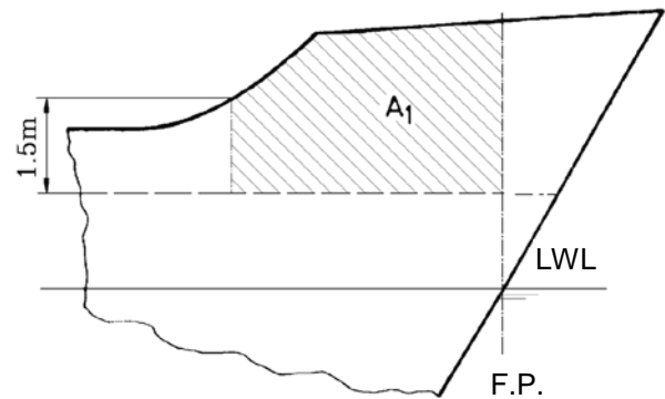
Figure 17.1 Effective area A_1 of bulwark
