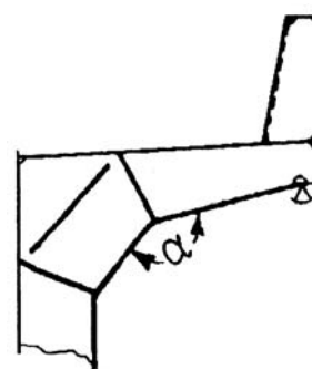
Figure 3.4 Support of face plates of cantilevers
