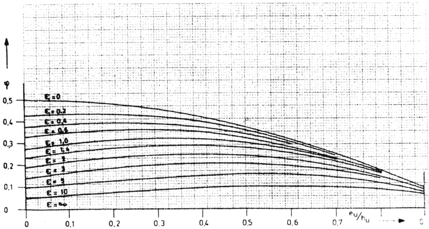
Diagram 8.2 coefficient \phi
