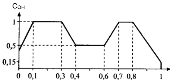
Figure 6.4 Distribution factor C_{QH}
