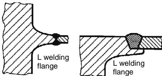
Figure 20.2 Welding flanges on steel castings of forgings
