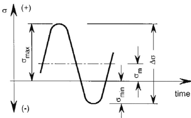
Figure 3.13 Dynamic load cycle
