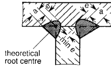
Figure 20.14 Filler welds with increased penetration
