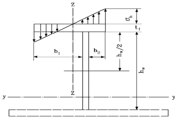
Figure 3.11 Asymmetrical profile
