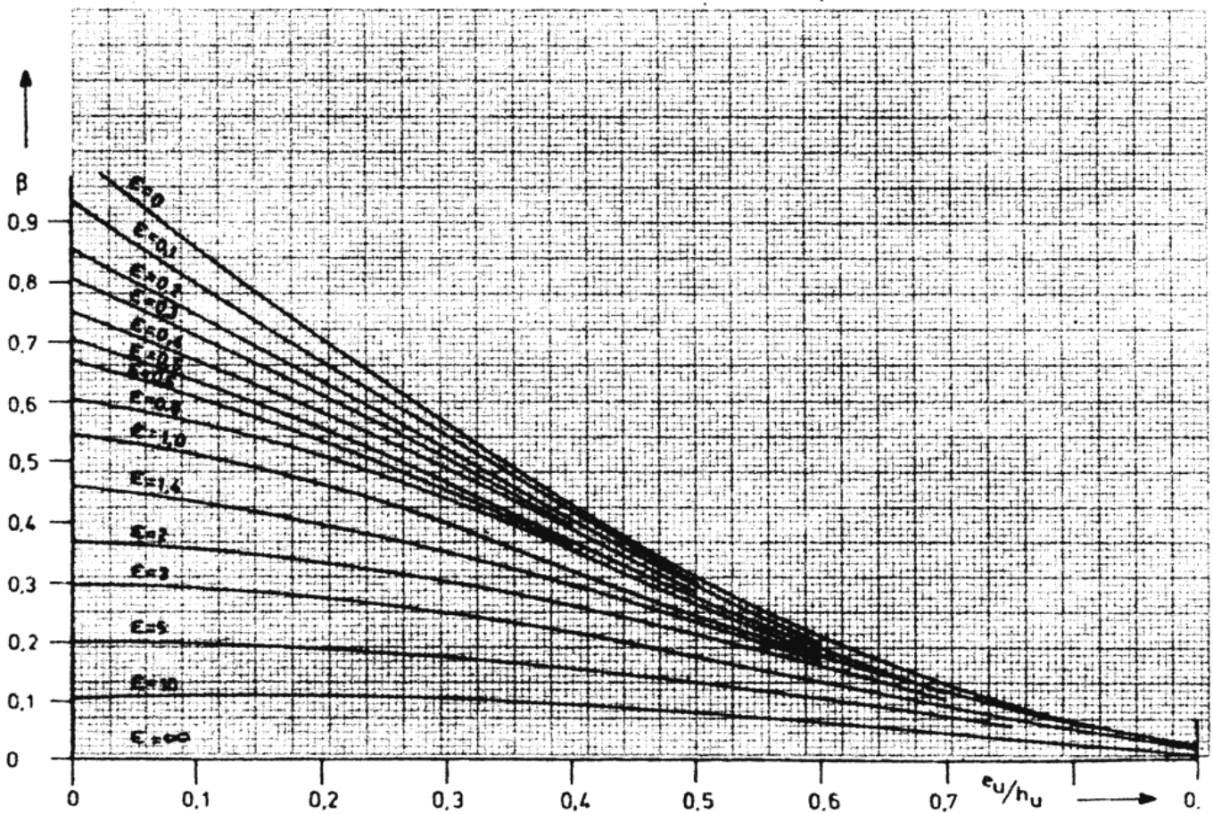
Diagram 8.3 coefficient \beta
