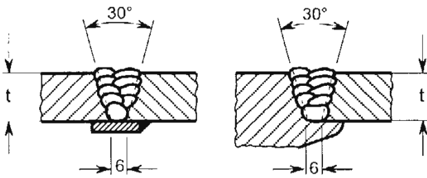
Figure 20.6 Single-side welds with permanent weld pool supports (backings)
