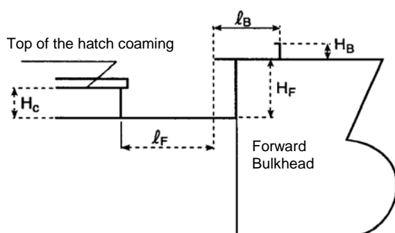
Figure 27.3 Dimensions of the forecastle
