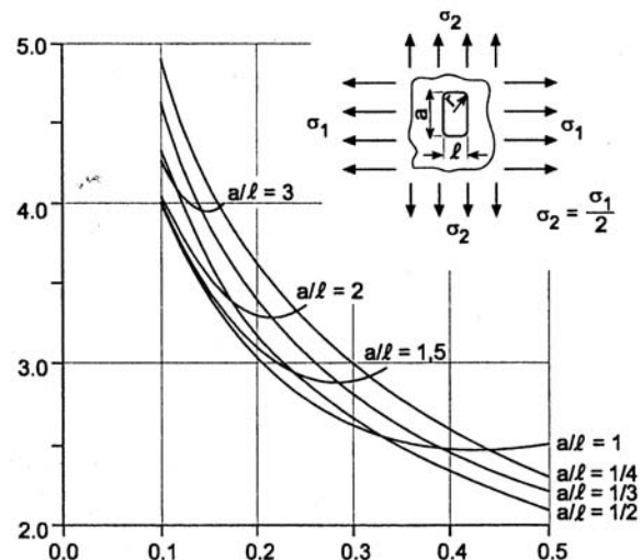
Figure 3.9 Notch factor K_t for rectangular openings with rounded corners at uniaxial state of stresses (left) and at multiaxial state of stress (right).
