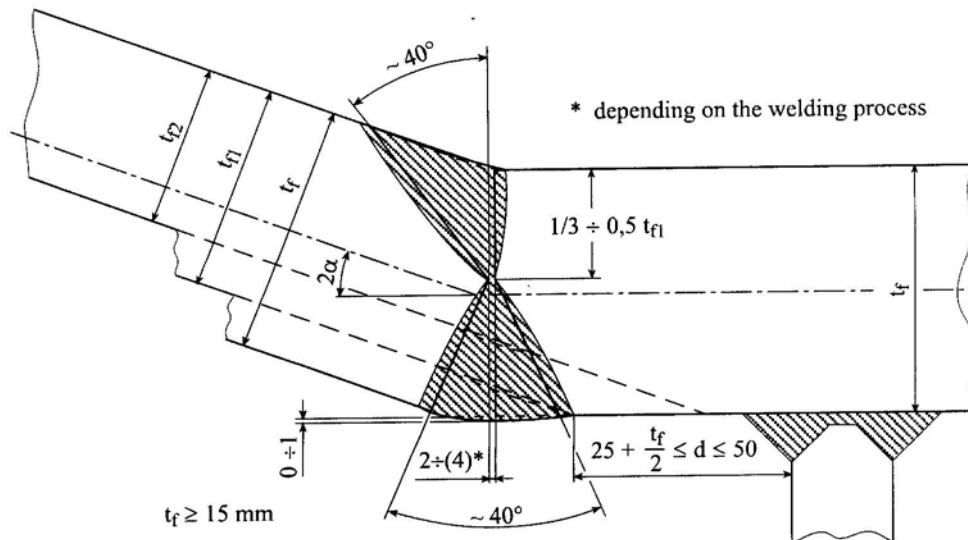
Figure 3.6 Welding and support of knuckles
