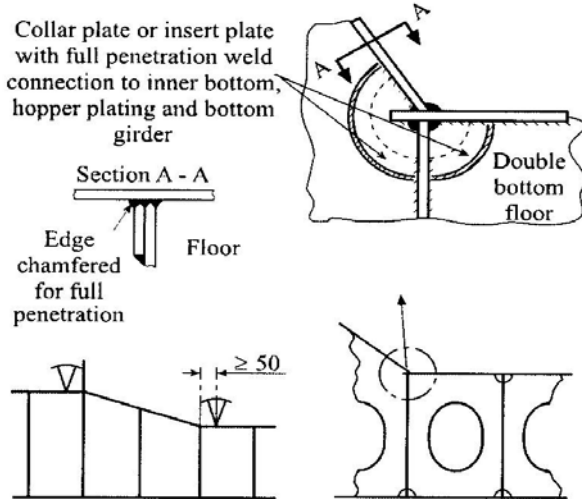
Figure 3.7 Knuckles of the double bottom
