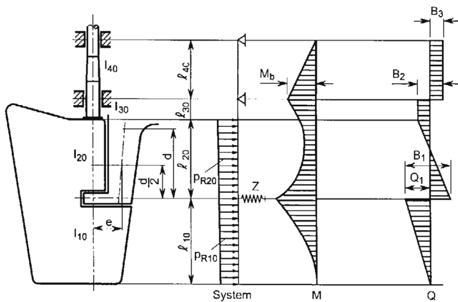
Figure 18.4 Semi-spade rudder
