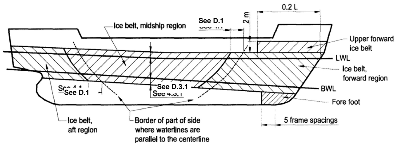
Figure 14.2 Ice belt
