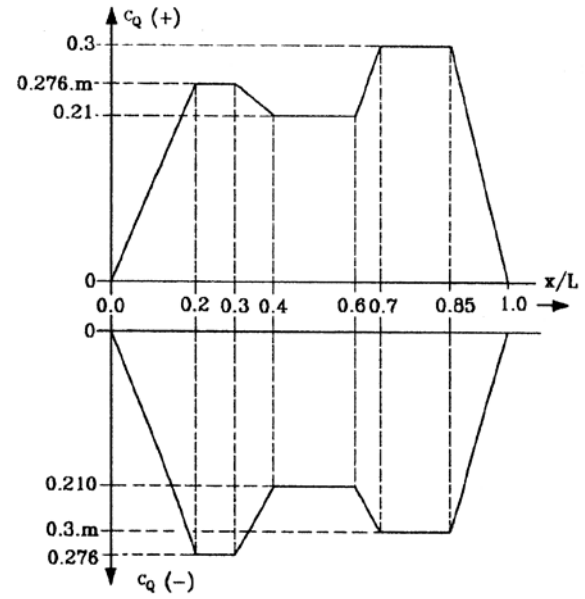
Figure 6.3 Distribution factor C_Q
