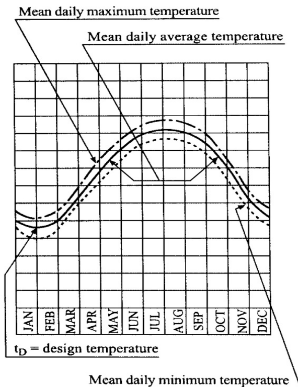
Figure 3.1 Commonly used definitions of temperatures
