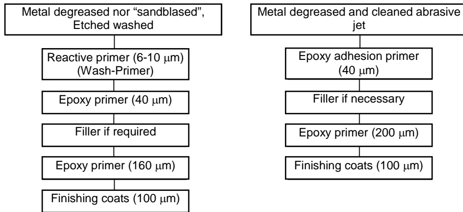
Figure 22.1 Typical coating systems for aluminum structures
