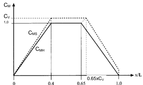
Figure 6.2 Distribution factor C_M and influence factor C_V
