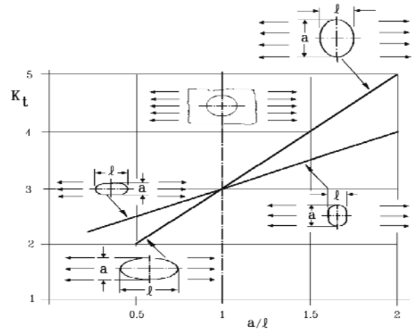
Figure 3.8 Notch factor K_t for rounded openings
