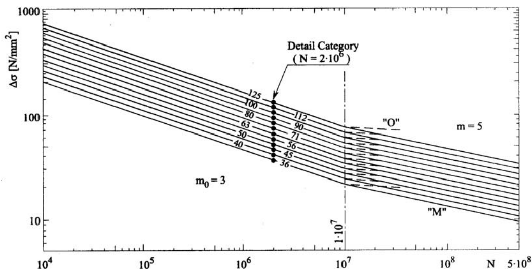
Figure 3.15 "S-N" curves for welded joints at steel
