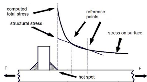
Figure 3.17 Structural stress
