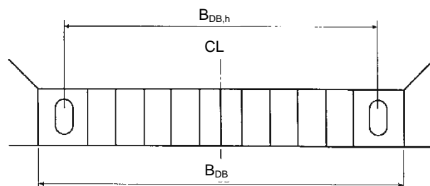
Figure 27.10 Effective distances BDB and BDB,h for the calculation of shear capacity
