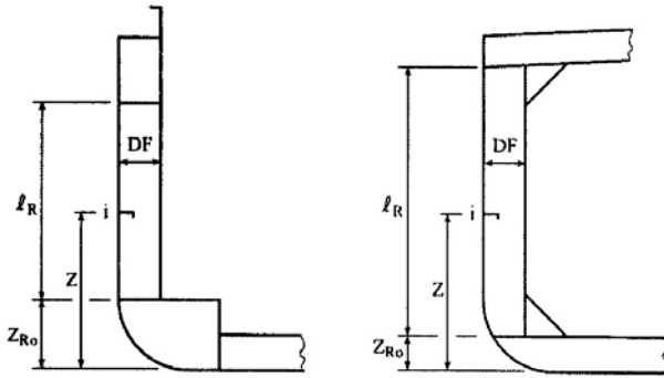
Figure 8.6 Definitions
