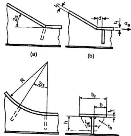
Figure 3.5 Typical stiffeners of rounded or knuckled face plates
