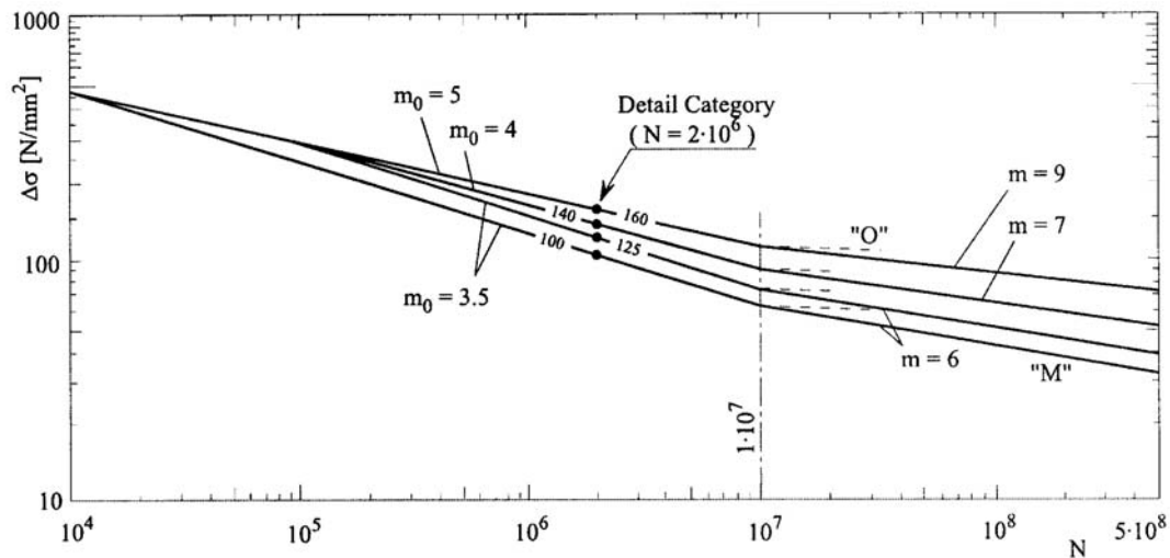
Figure 3.16 "S-N" curves for notches at plate edge of steel plate
