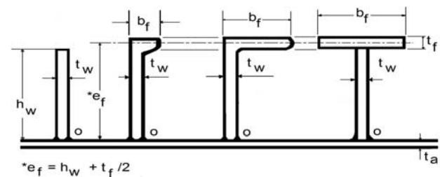
Figure 3.12 Main dimensions of typical longitudinal stiffeners
