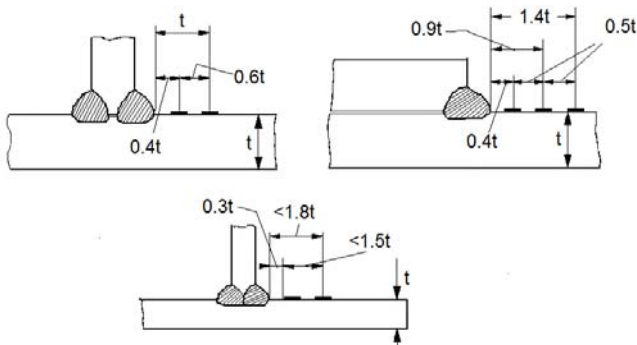
Figure 3.18 Strain gauges in plate structures
