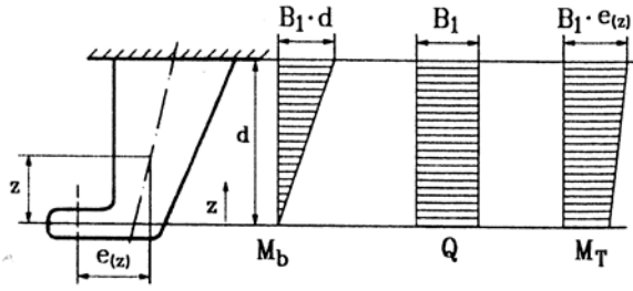
Figure 10.6 Loads on the rudder horn
