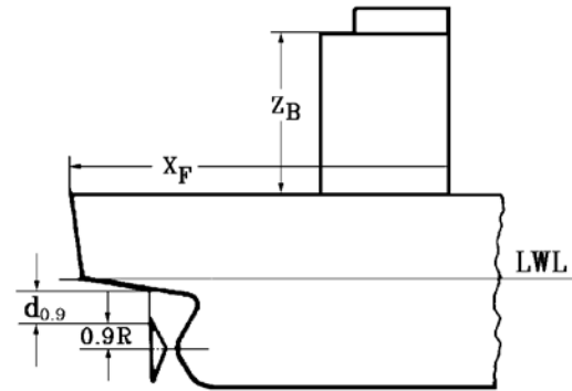
Figure 10.1 Propeller clearance d_{0.9}
