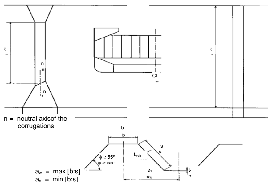
Figure 27.12a Span \ell of the corrugation (longitudinal section)
