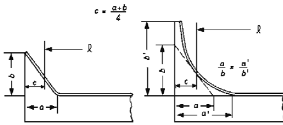
Figure 3.2 Unsupported span \ell
