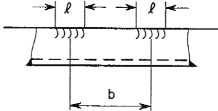
Figure 20.26 Intermittent fillet weld joint
