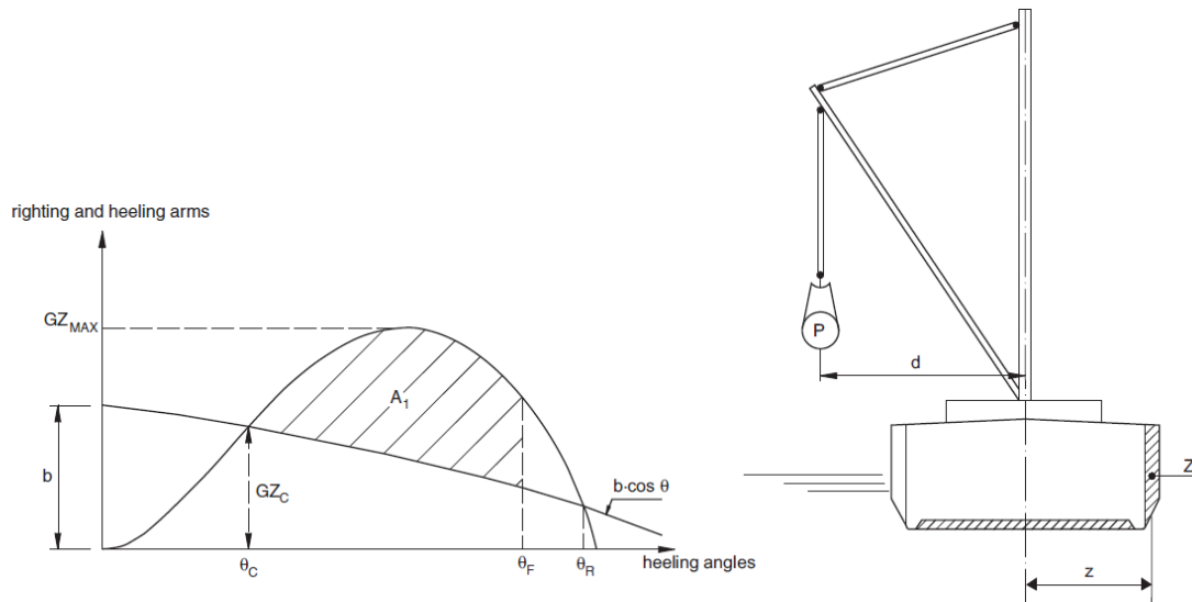
Figure 26.2 Cargo Lifting
