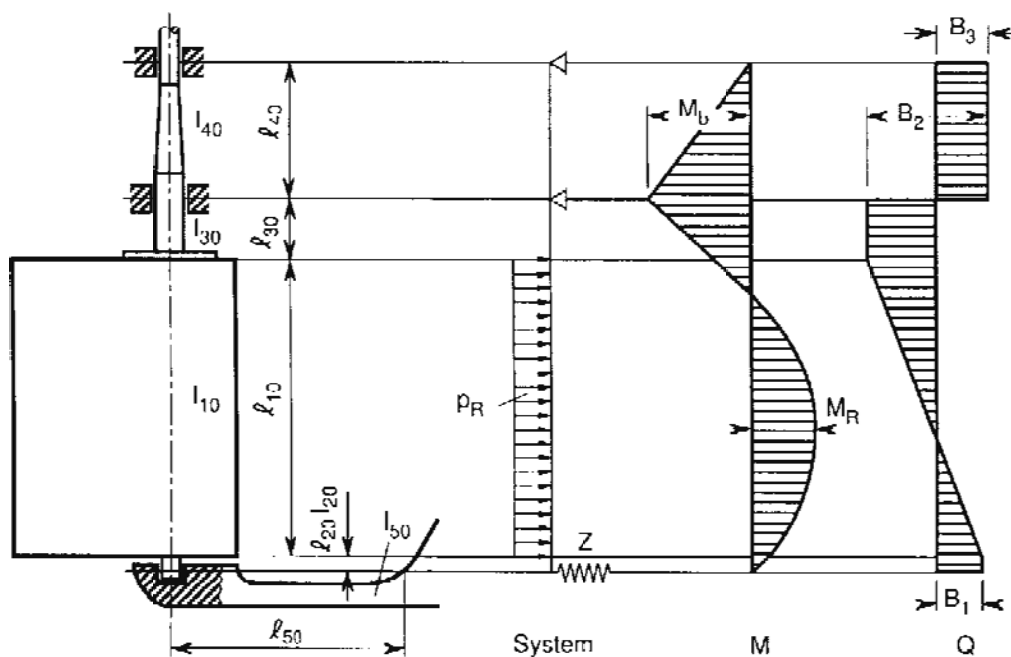
Figure 18.3 Rudder supported by sole piece
