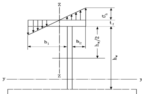
Figure 3.12 Asymmetrical profile
