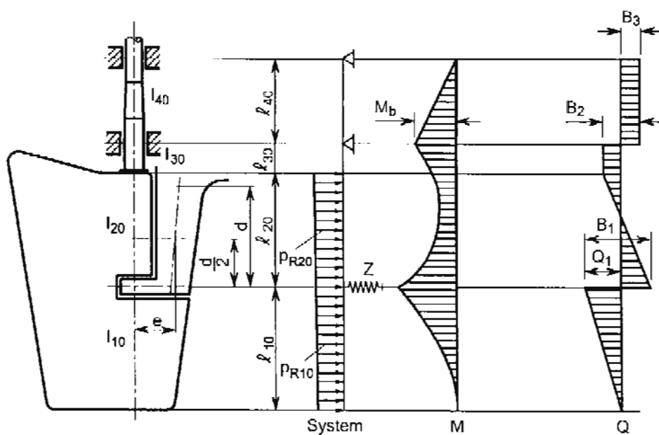
Figure 18.4 Semi-spade rudder
