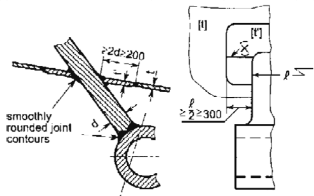
Figure 20.18 Shaft bracket with integrally cast welding flanges
