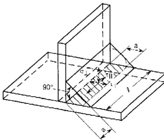
Figure 20.22 Stresses in a fillet weld
