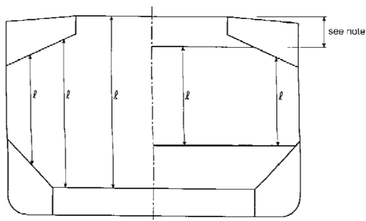
Figure 27.12a Span \ell of the corrugation (longitudinal section)
