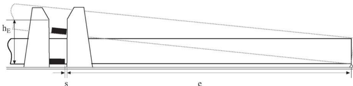
Fig. 15.10 Height of transverse cover guides
