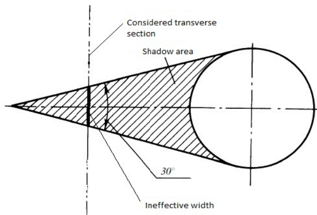
Figure 6.7 Shadow area
