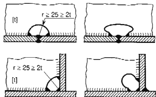
Figure 20.3 Welding out-outs
