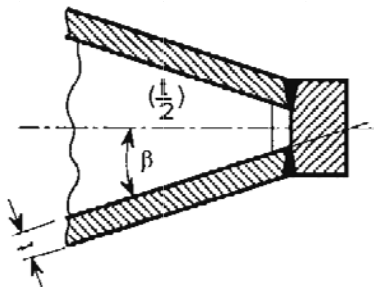
Figure 14.5 Stem
