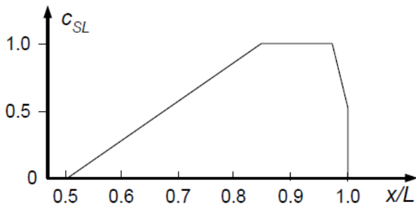
Figure 5.6 Distribution factor C_{SL}
