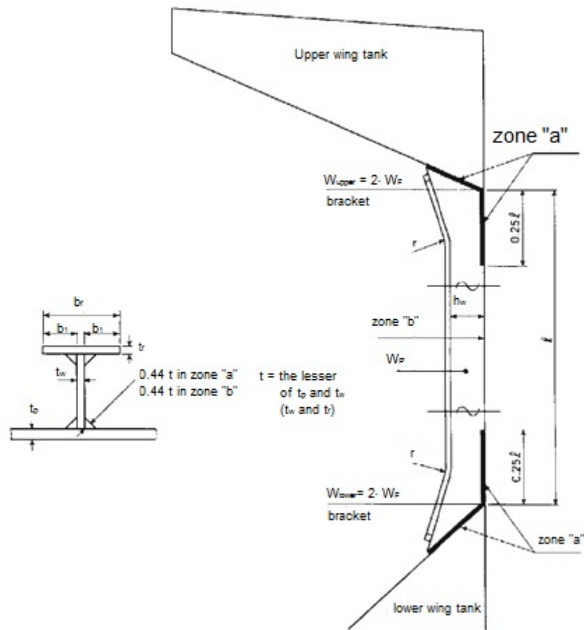
Figure 27.4 Side frame of single side skin bulk carrier
