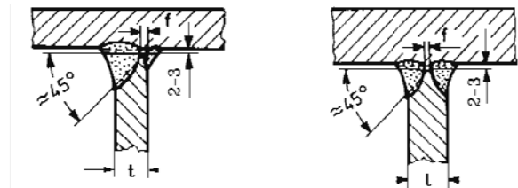
Figure 20.9 Single and double-bevel welds with defined incomplete root penetration
