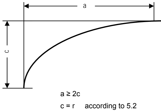
Figure 7.3 Elliptic or parabolic hatch corner
