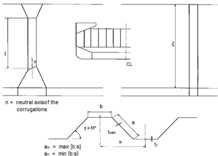
Figure 27.12a Span \ell of the corrugation (longitudinal section)
