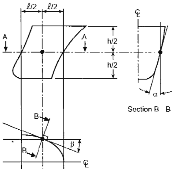
Figure 23.1 Definitions of angle \alpha and \beta
