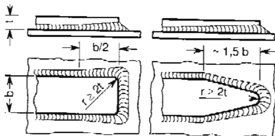
Figure 20.4 The ends of doubling plates
