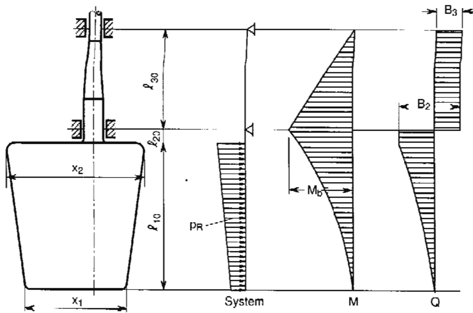
Figure 18.5 Spade rudder
