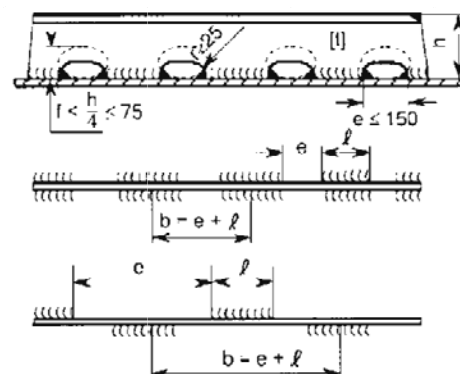
Figure 20.15 Scallop, chain and staggered welds
