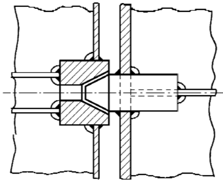
Figure 23.3 Thrust bearing
