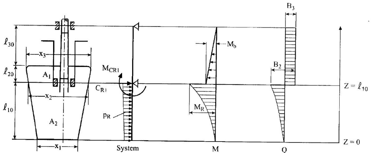
Figure 18.5 Spade rudder
