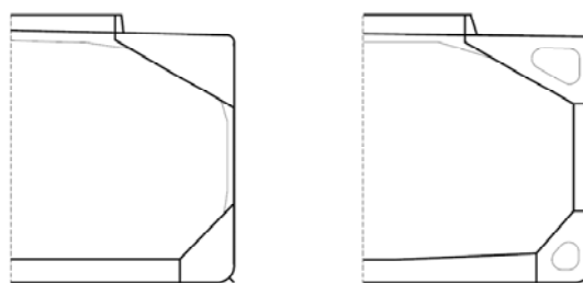
Fig 27.2 Single and double skin bulk carrier
