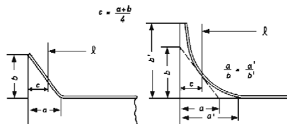
Figure 3.3 Unsupported span \ell
