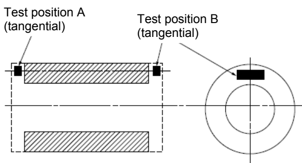
Fig. 5.8 Hollow pinion
