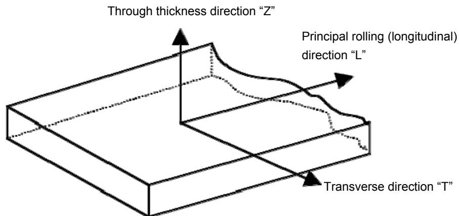
Figure 3.8 Schematic of testing directions
