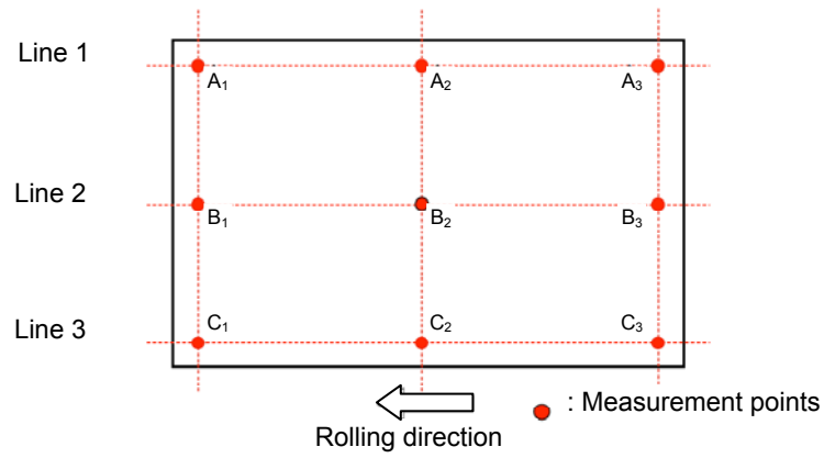
Figure 3.1a - Locations of thickness measuring points for the original steel plates
