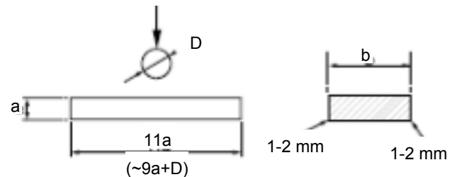
Figure 2.7 Flat bend test specimen
