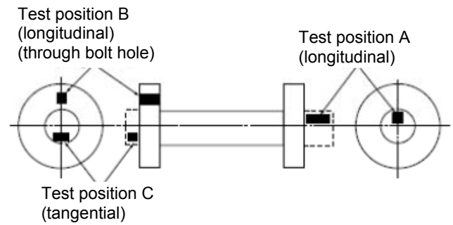
Figure 5.2 Flanged shaft
