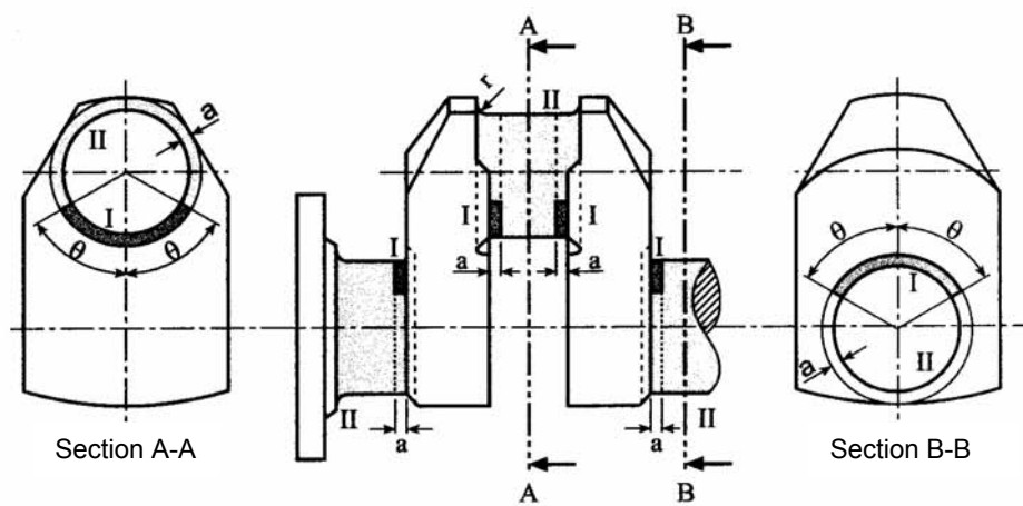
(a) Solid crankshaft
