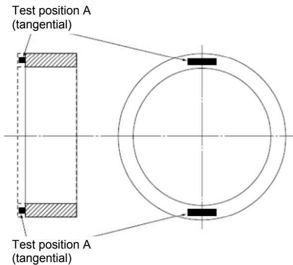
Fig. 5.7 Wheel rim
