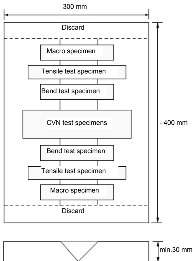
Figure 11.B.1 Weld test assembly
