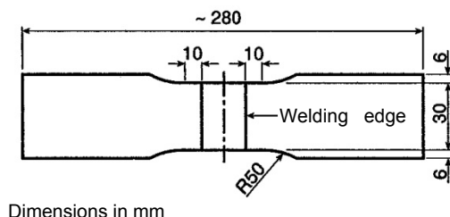
Figure 11.A.3 Tensile test specimen
