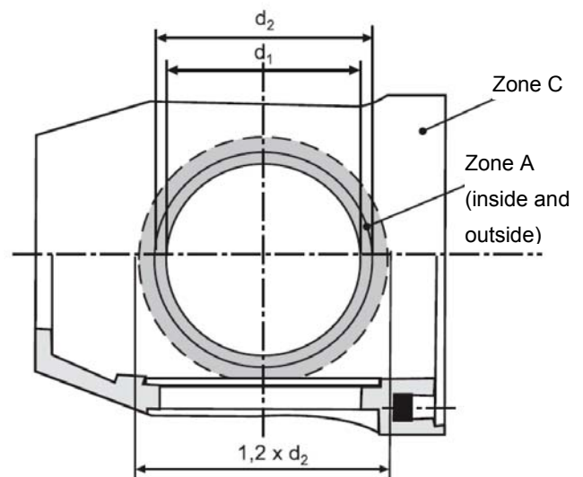
Figure 11.5 Severity zones for controllable pitch propeller boss
