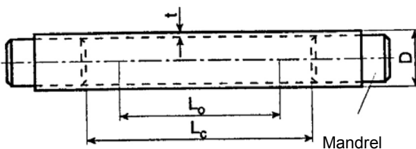
Figure 2.3 Full cross-section specimen
