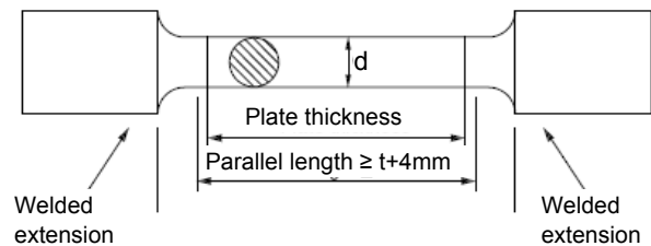
Figure 3.11 Welded test specimen
