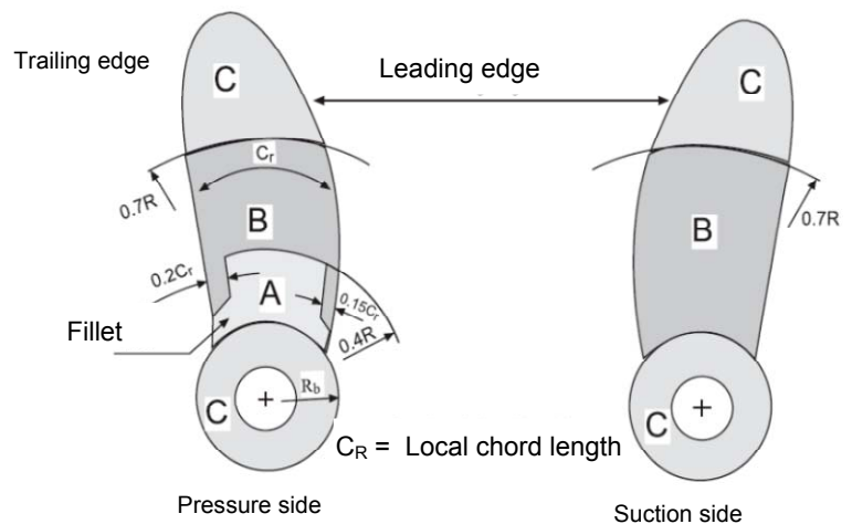
Figure 11.3 Severity zones for integrally cast low-skew propellers
