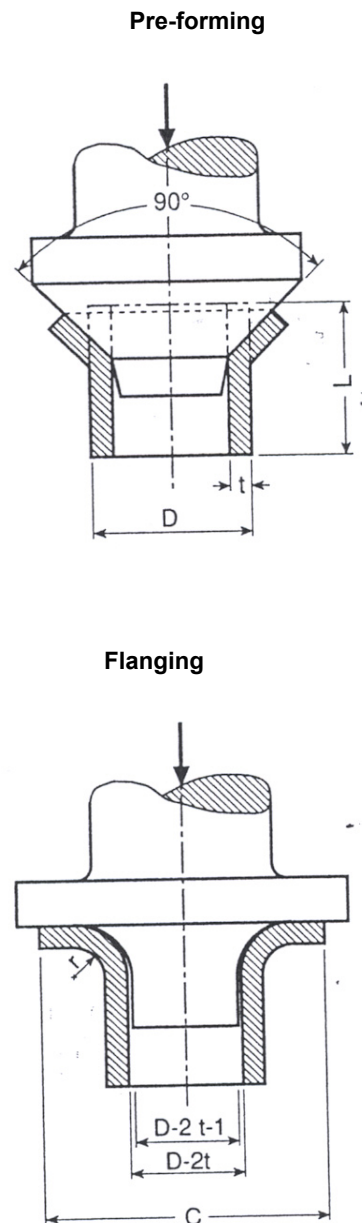
Figure 2.11 Flanging test
