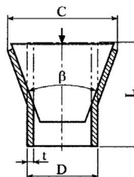
Figure 2.10 Drift expanding test
