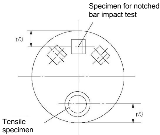
Figure 10.7 Sampling of steel bars, forgings and castings
