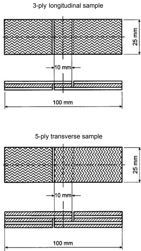
Fig. 12.1 Typical representation of a 3-ply longitudinal and a 5-ply transverse tensile lap-shear sample
