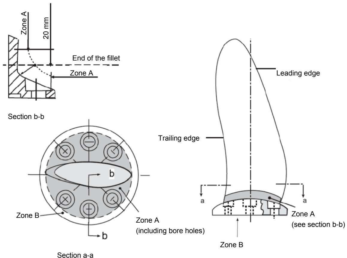
Figure 11.6 Severity zones for controllability pitch and built-up propeller
