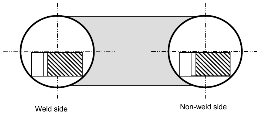
Figure 10.6 Location of CTOD test specimens
