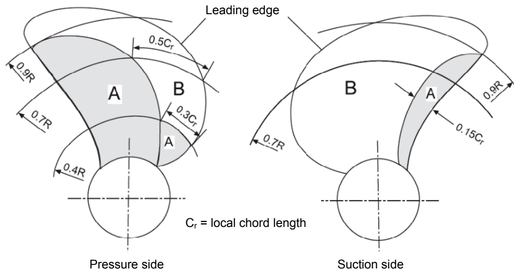
Figure 11.4 Severity zones in blades with skew angles greater than 25 °
