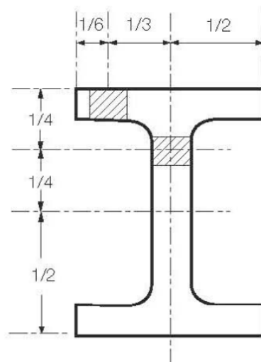
Figure 3.6 H-Section
