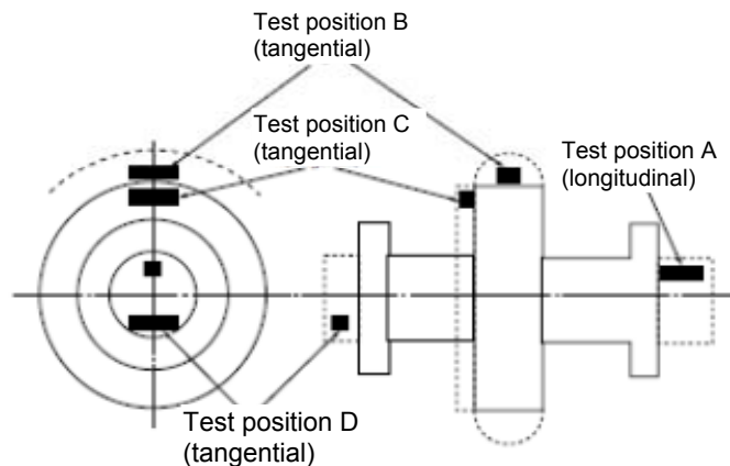
Figure 5.3 Flanged shaft with collar
