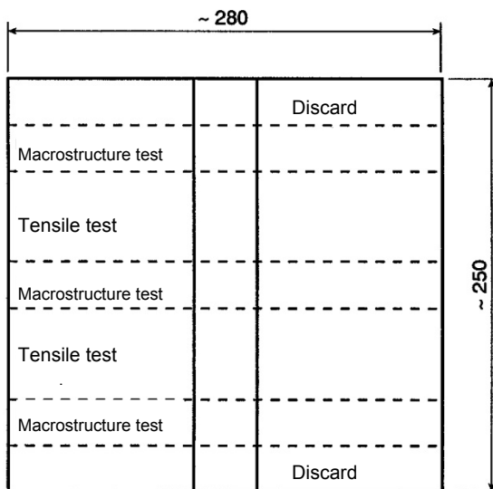
Figure 11.A.1 Test piece
