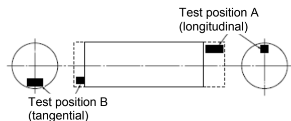
Figure 5.1 Plain shaft
