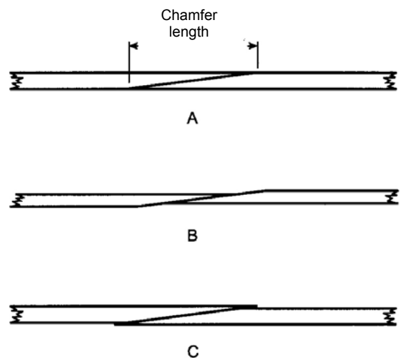
Figure 12.8 Scarf joints across the thickness
