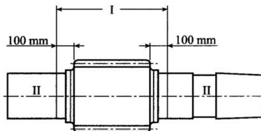
Pinion shafts
