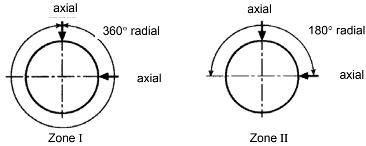
Scanning directions for Type A ve Type B
