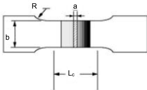
Figure 2.6 Specimen for tensile test on butt weld
