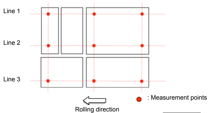
Figure 3.1b - Locations of thickness measuring points for the cut steel products
