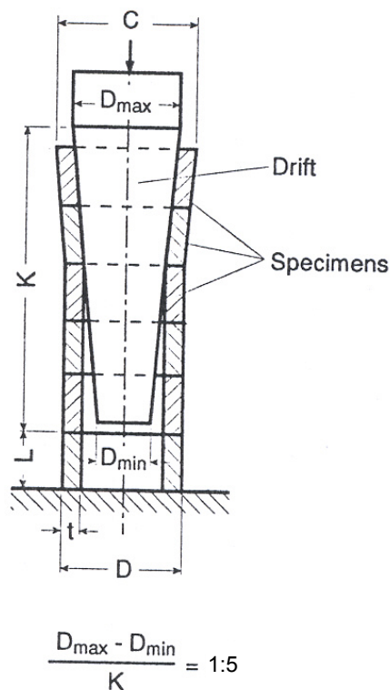
Figure 2.12 Ring expanding test
