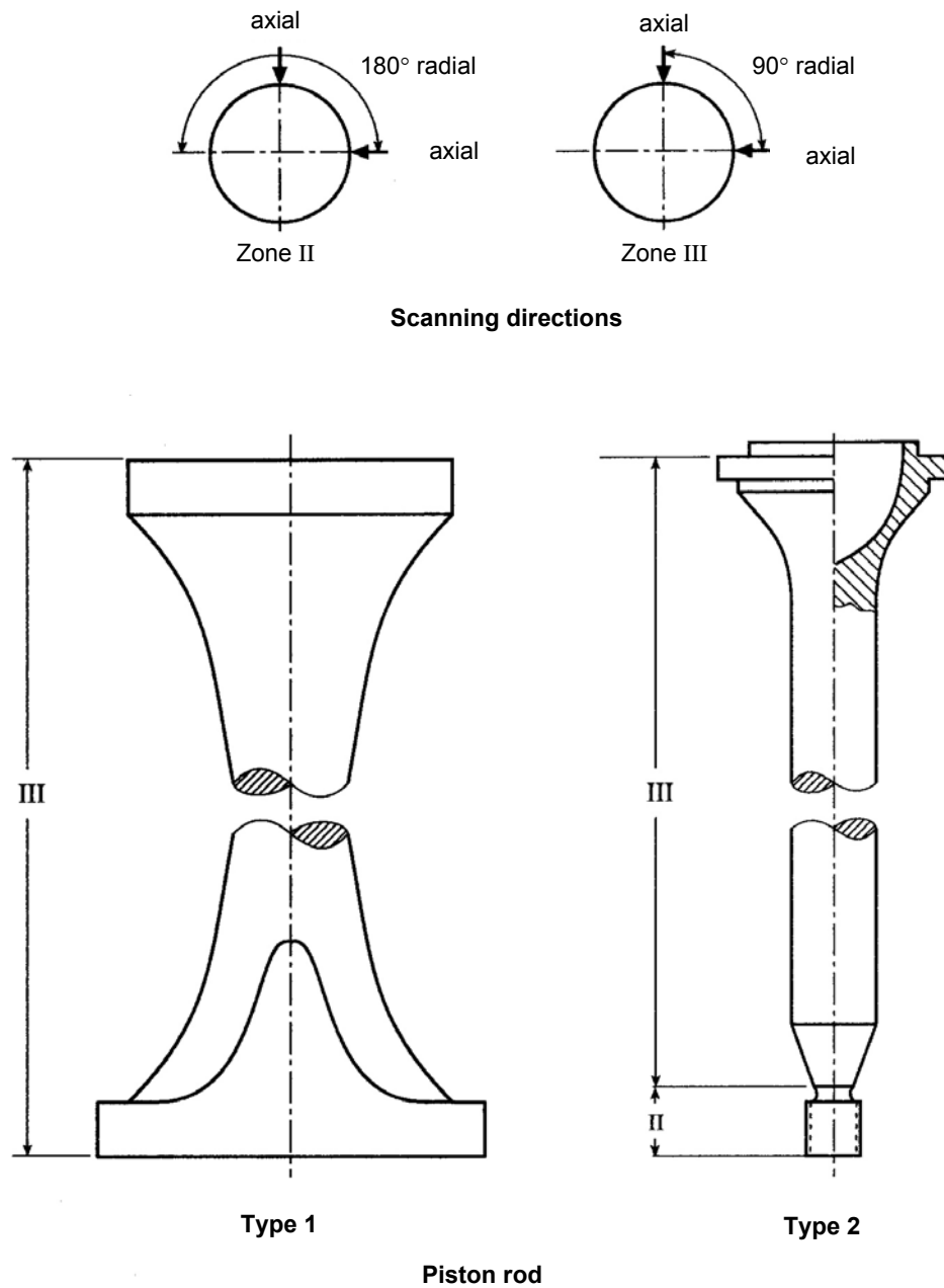
Fig. 5.19 Inspection zones for ultrasonic testing of machinery components
