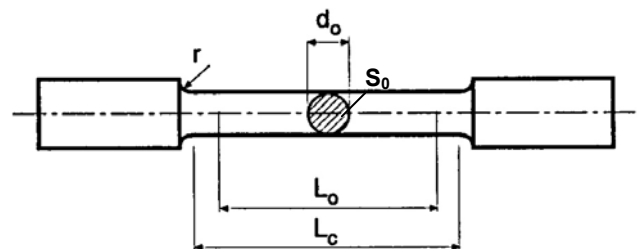
Figure 2.1 Round specimen
