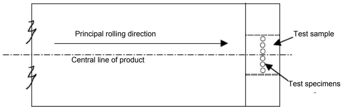
Figure 3.9 Plate and wide flat sampling position
