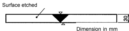
Figure 11.A.2 Macrostructure test specimen
