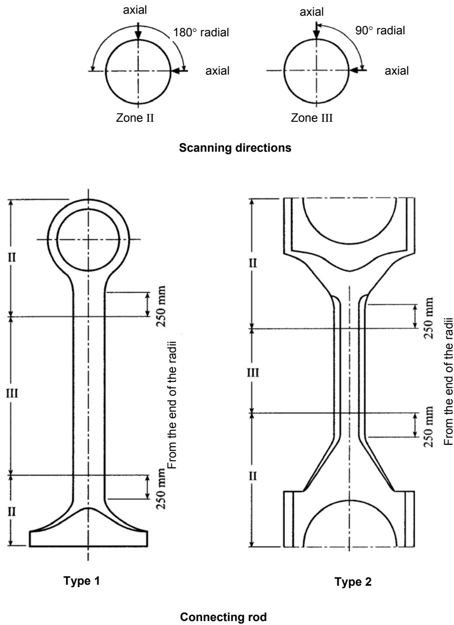
Fig. 5.20 Inspection zones for ultrasonic testing of machinery components
