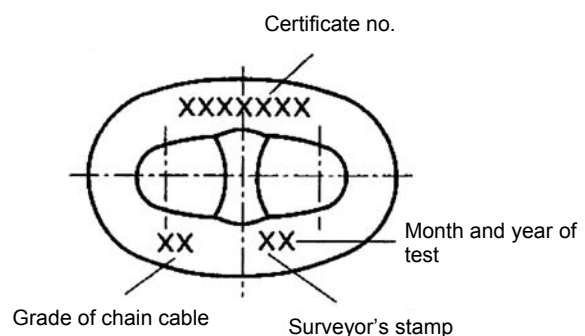
Figure 10.4 Marking of chain cables
