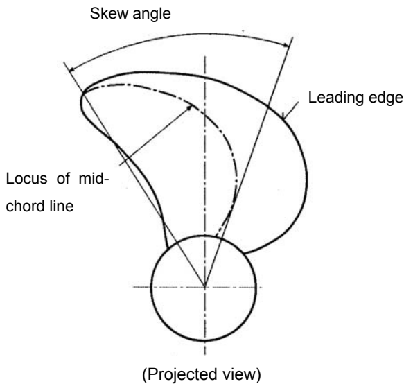
Figure 11.2 Definition of skew angle
