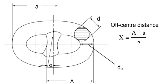
Figure 10.3 Manufacturing tolerances
