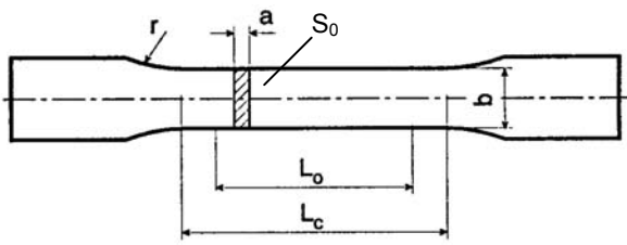
Figure 2.2 Flat specimen
