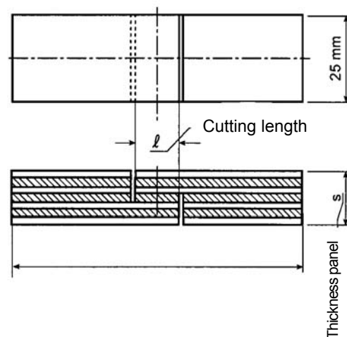
Fig. 12.4 Longitudinal sample for a 7-ply plywood panel
