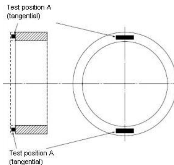
Fig. 5.7 Wheel rim
