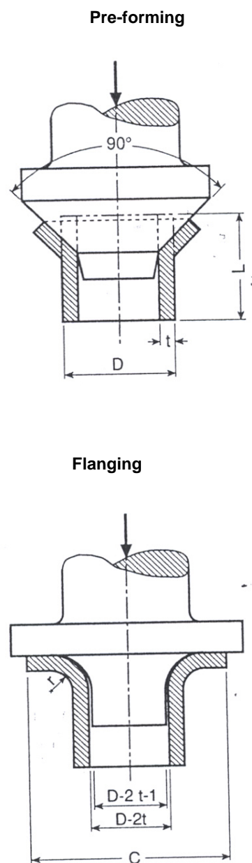
Figure 2.11 Flanging test
