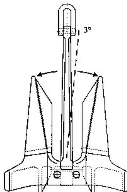
Figure 10.1 Allowable lateral movement of shank
