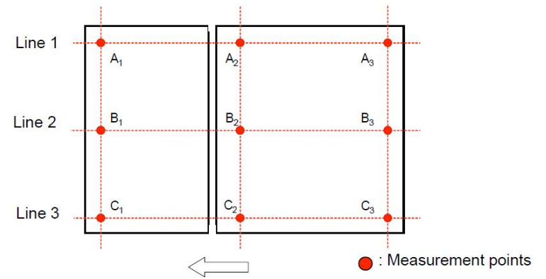
Figure 3.1a - Locations of thickness measuring points for the original steel plates
