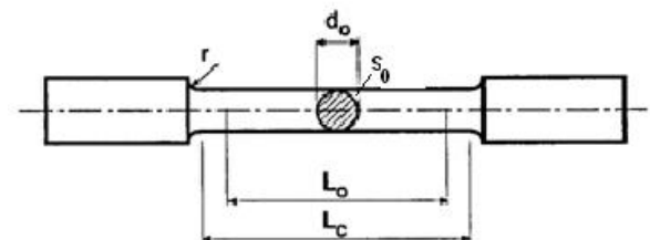
Figure 2.1 Round specimen
