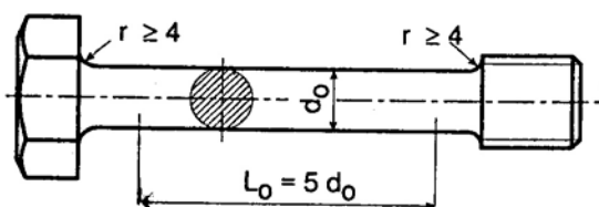
Figure 14.1 Turned specimen
