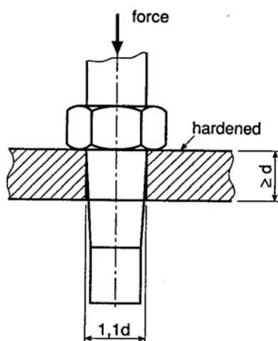
Test arrangement
