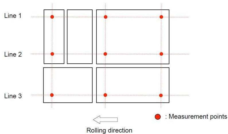
Figure 3.1b - Locations of thickness measuring points for the cut steel products
