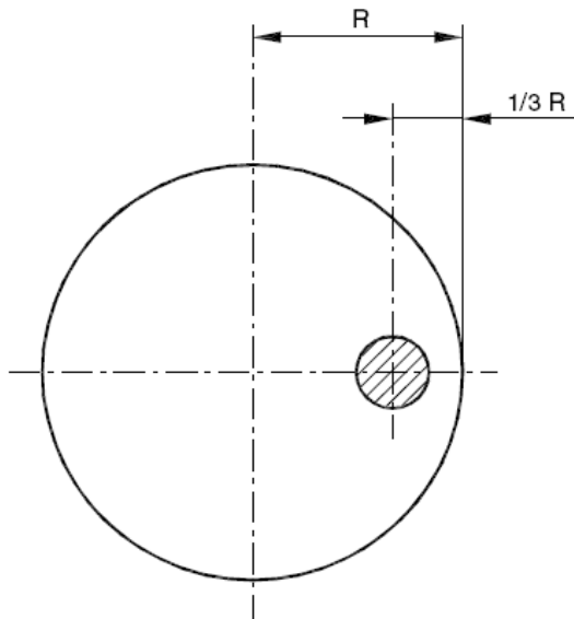
Figure 3.7 Bars
