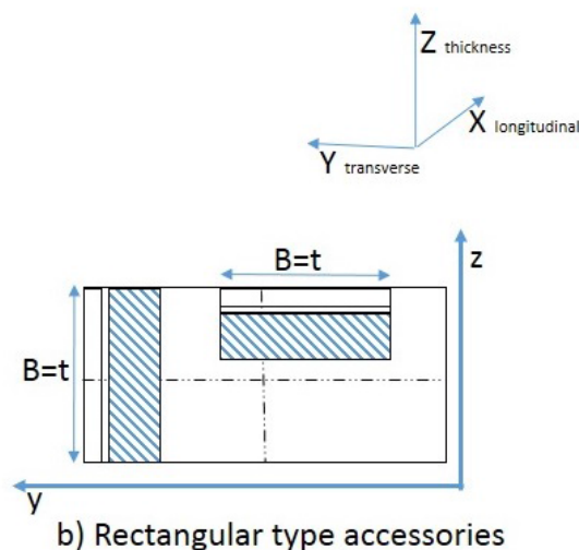
Figure 10.7 Location of CTOD test specimens: a) Circular type accessory and b) rectangular type accessory, B corresponds to the thickness of material, the grain flow is considered in the longitudinal direction X
