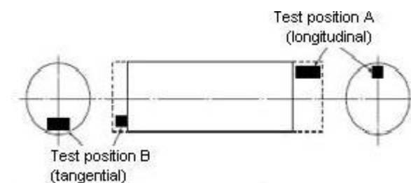
Figure 5.1 Plain shaft
