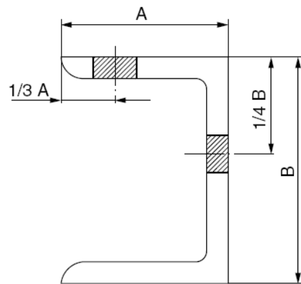
Figure 3.5 Channel
