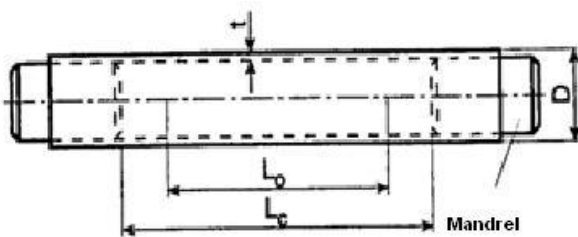
Figure 2.3 Full cross-section specimen
