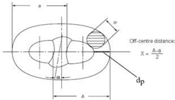
Figure 10.3 Manufacturing tolerances
