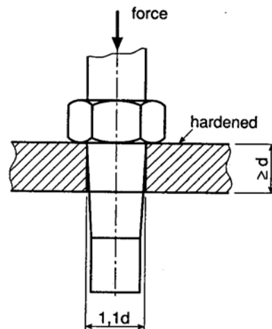
Test arrangement
