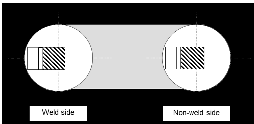
Figure 10.6 Location of CTOD test specimens for chain
