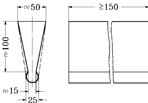
Figure 9.2 Sample piece
