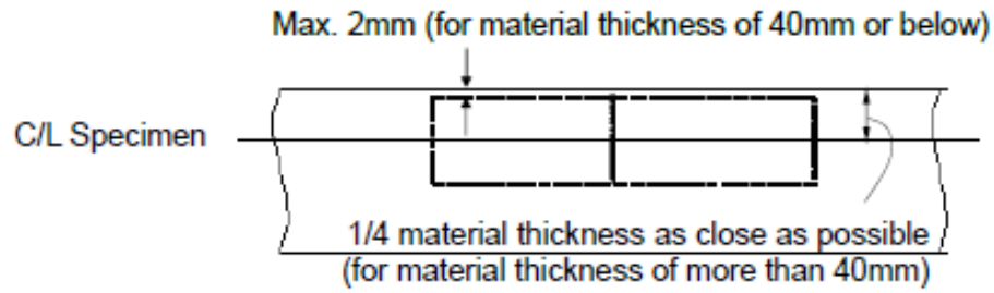
Figure 3.7a Sampling position of Charpy V-notch impact test specimens (Base metal)
