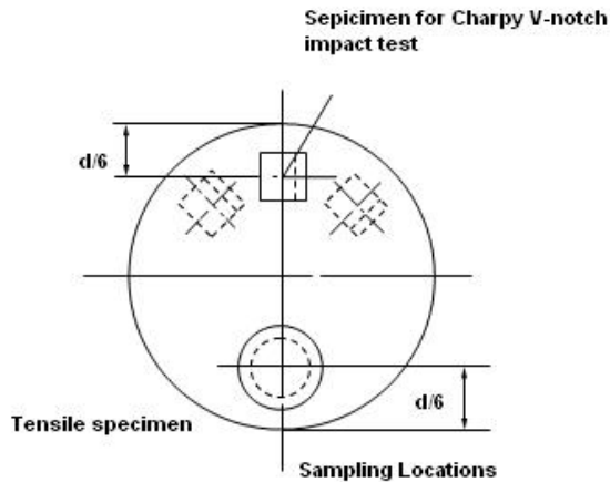
Figure 10.2 Sampling locations
