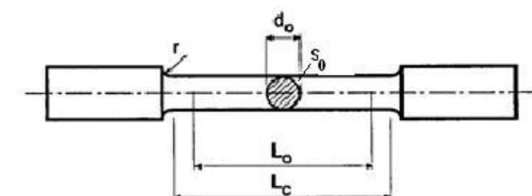
Figure 2.1 Round specimen
