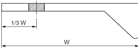
Figure 3.3 Bulb flats
