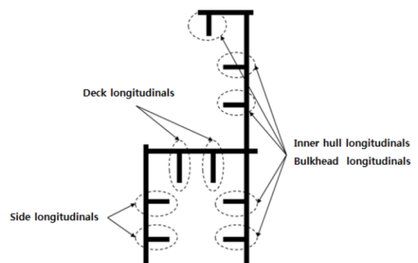
Figure 3.14 Upper Flange Longitudinal Structural Members
