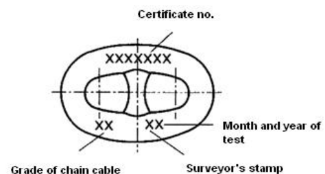
Figure 10.4 Marking of chain cables
