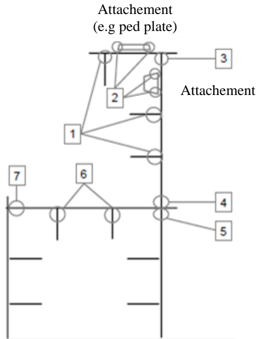
Figure 3.15 Other Weld Areas
