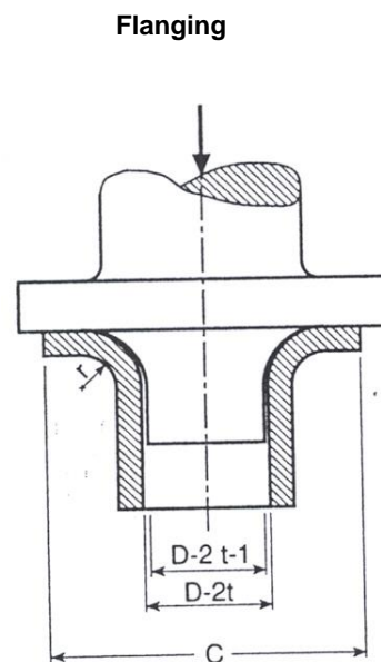
Figure 2.11 Flanging test
