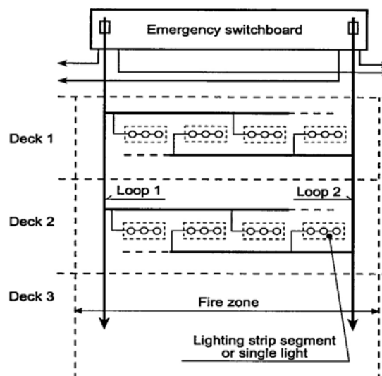
Fig. 14.1 Specimen of supply layout-low-location lighting
