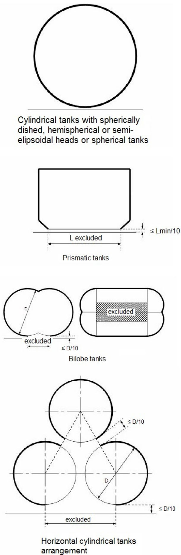
Figure 8.1 External surface area of the tank for different tank types
