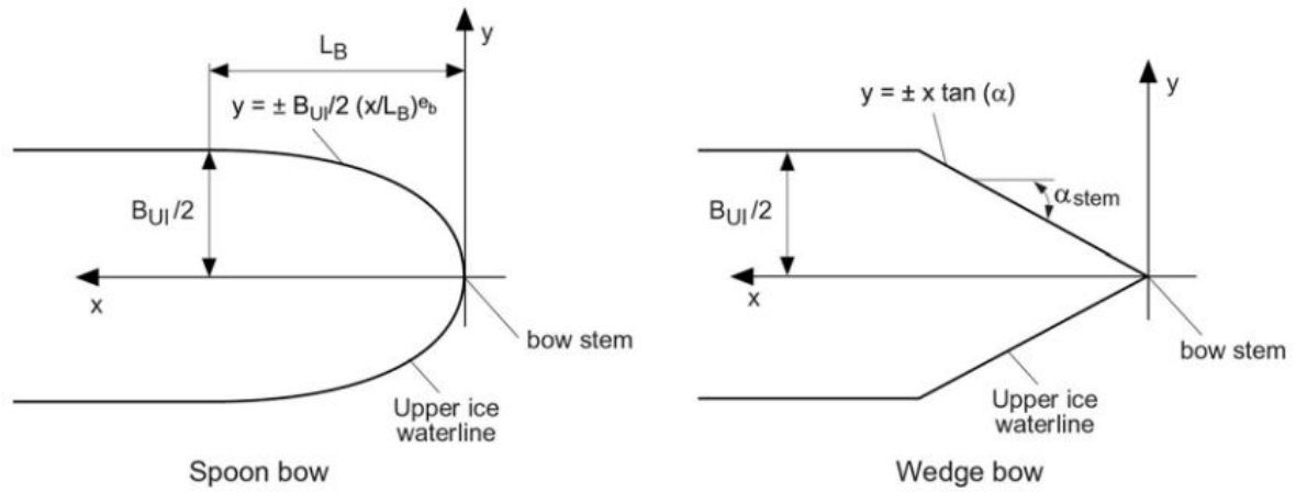
Figure 10 - Bow Shape Definition
