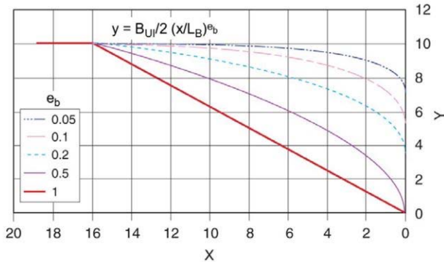
Figure 10 - Bow Shape Definition
