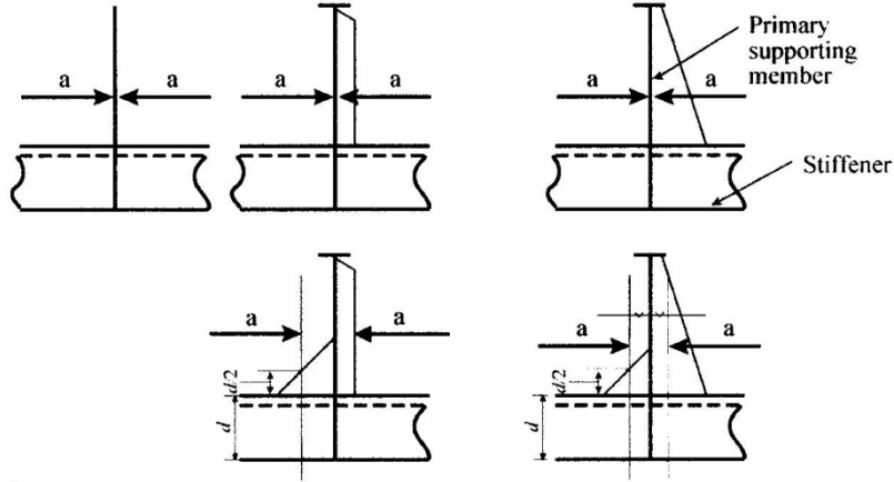
Figure 6 - Design span of framing member
