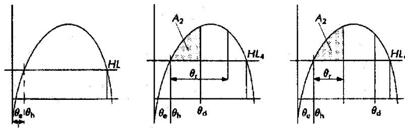
Figure 2 - Damage stability
