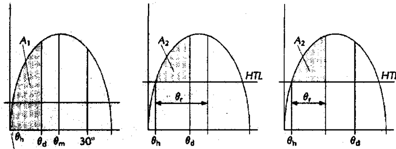
Figure 1 - Intact stability
