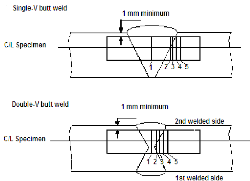
Figure 16.2 – Orientation of weld test specimen
