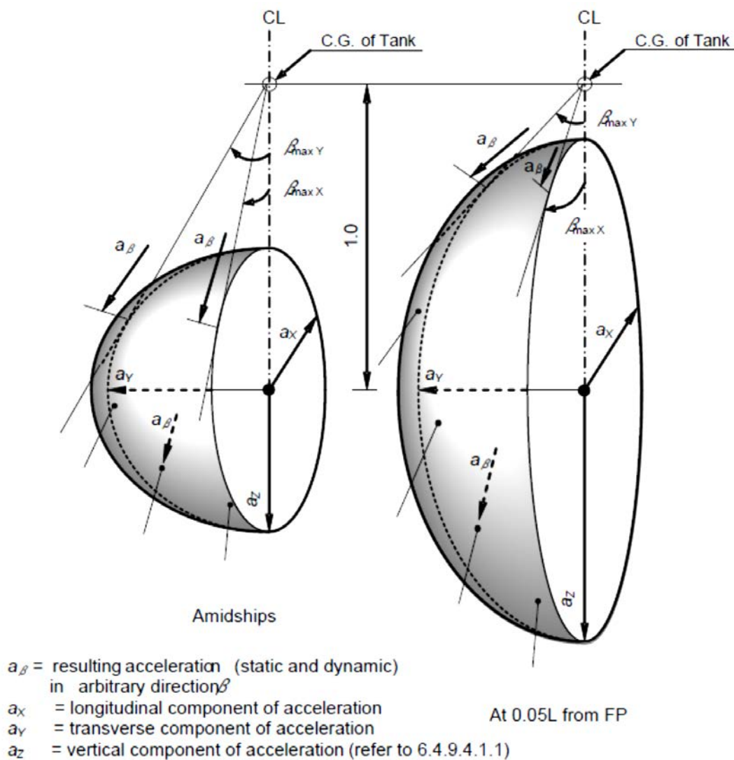
Figure 6.4.1 – Acceleration ellipsoid
