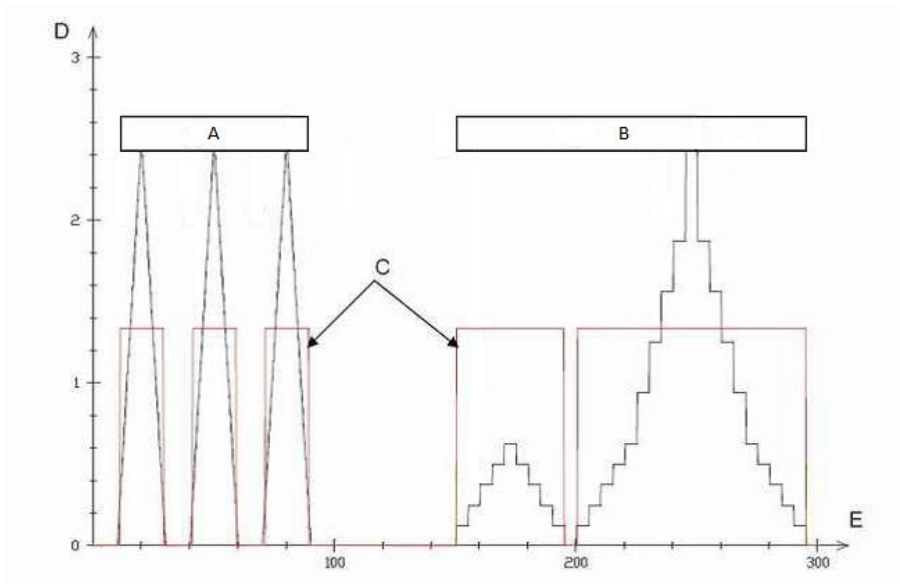
Key A Static tests B Dynamic tests C Area for measurements D Applied voltage [V] E Time [s]
